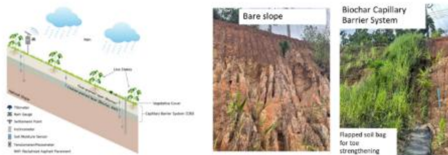
Figure 1: Biochar capillary barrier system
