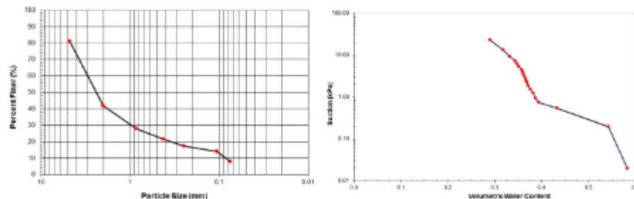
Figure 2: PSD and SWCC of biochar
